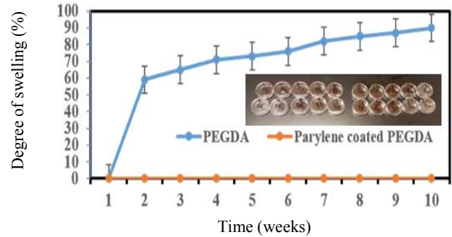
Fig. 2. Hydrolytic degradation test of PEGDA sample coated with parylene.
