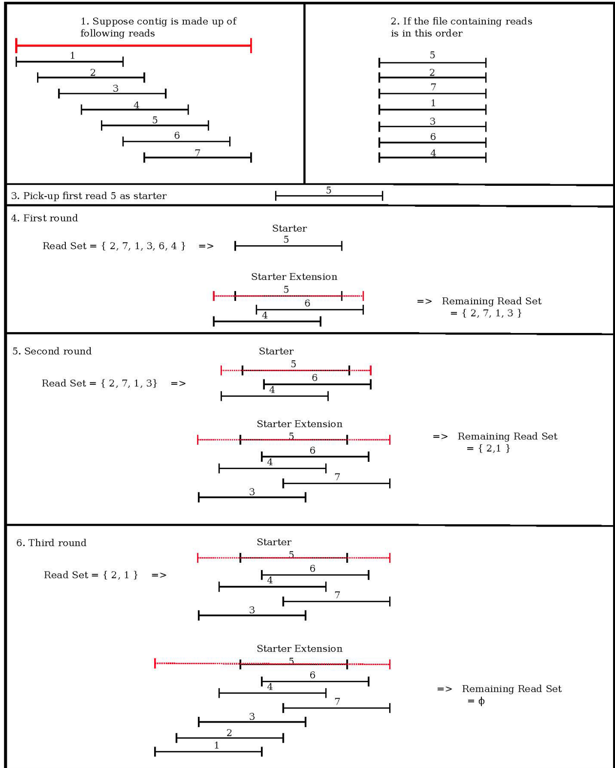
Figure 3 Example showing construction of contig using our approach (see online version for colours)
