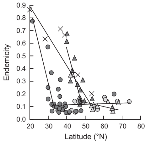
Figure 5. Regional endemism as a function of latitude for Atlantic (circles), Pacific (crosses) and European (triangles) realms: dark fill unglaciated areas light fill glaciated areas. Lines for the Atlantic and European realms were fitted by piecewise regression.
