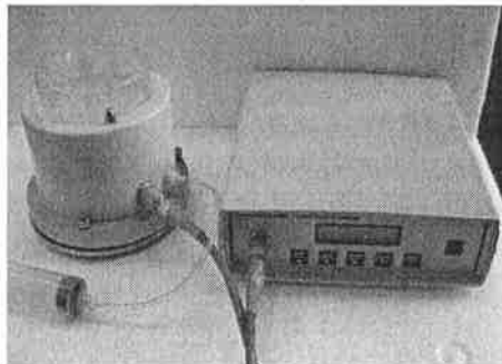
Figure 3. Autoclam permeability system
