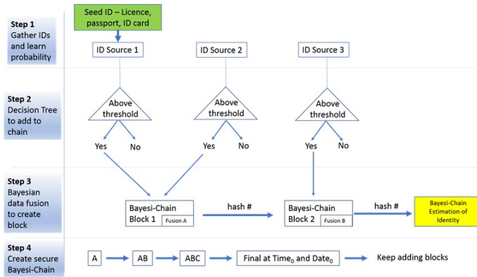
Figure 1: Bayesi-Chain Design Overview
