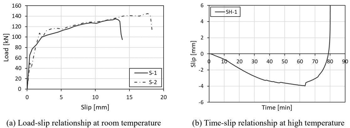
Fig. 5 Structural response of the solid slab specimens
