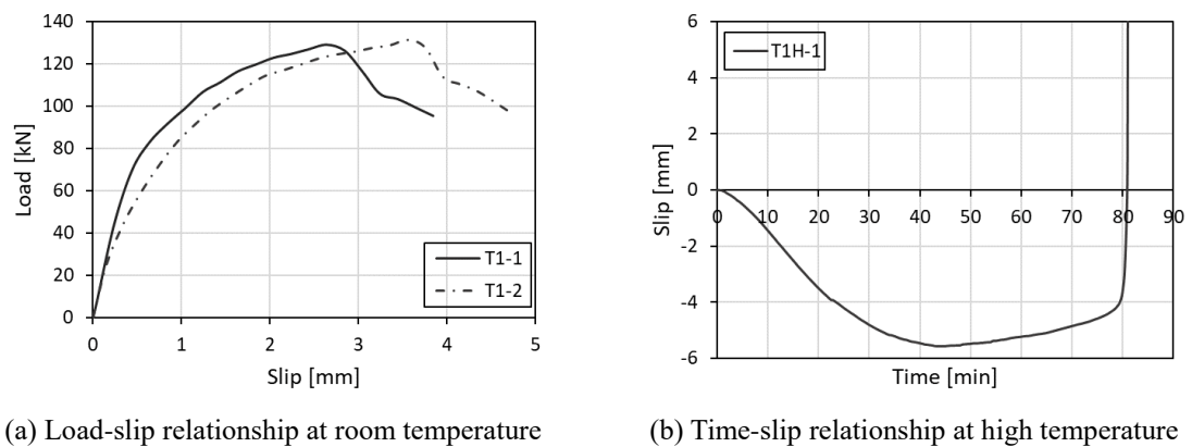
Fig. 6 Structural response of the transverse deck specimens with through-deck welding
