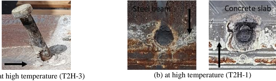
Fig. 10 Failure mode of the trapezoidal deck specimens with through-hole welding
