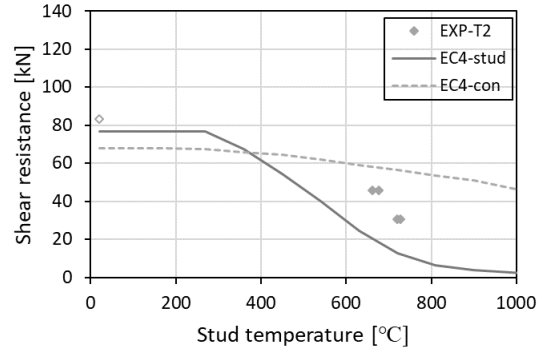
(b) 0.9t through-hole welded specimen
