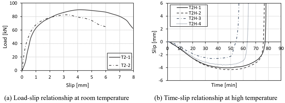
Fig. 7 Structural response of the transverse deck specimens with through-hole welding
