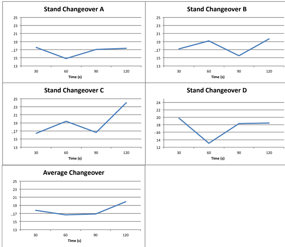
Figure 6 Power Signatures of each Stand Changeover for Batch 1
