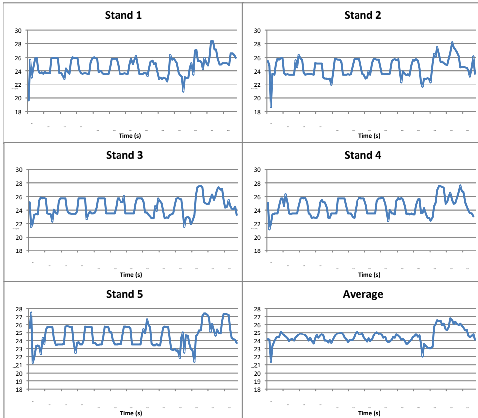
Figure 5 Power Signature of Each Stand for Batch 1
