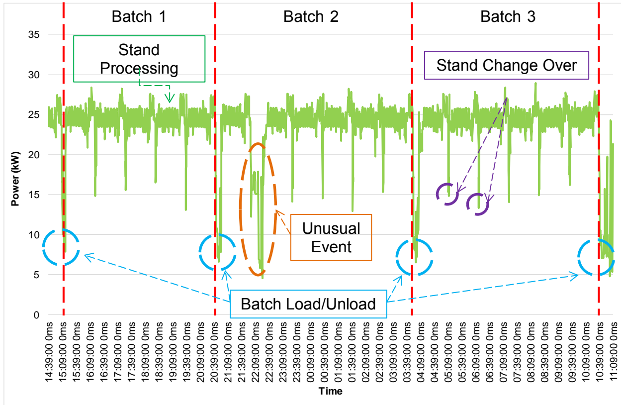
Figure 3 GRND01- Power logged while manufacturing 3 batches
