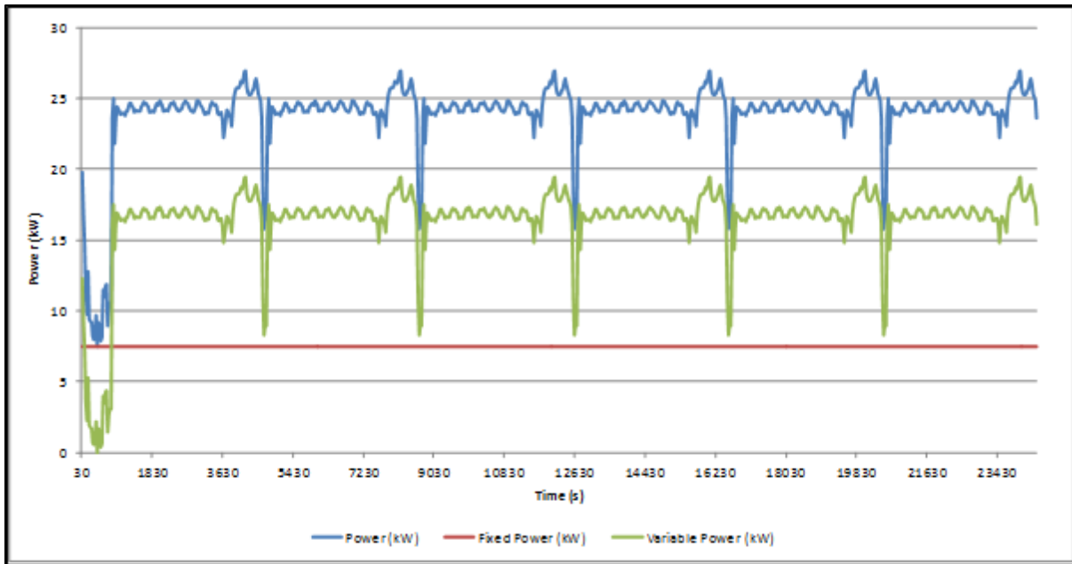
Figure 7 Final Power Profile for GRND01 with a Full Batch (12 Parts)
