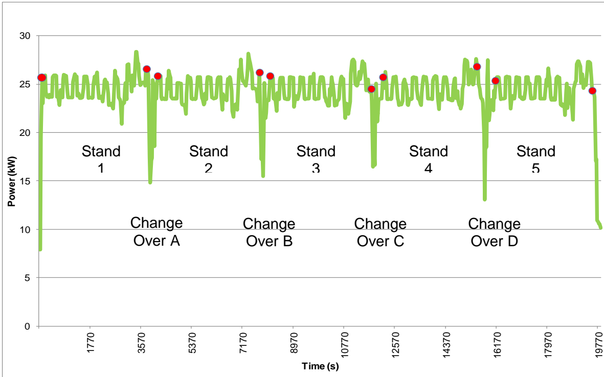
Figure 4 GRND01 Power Signature
