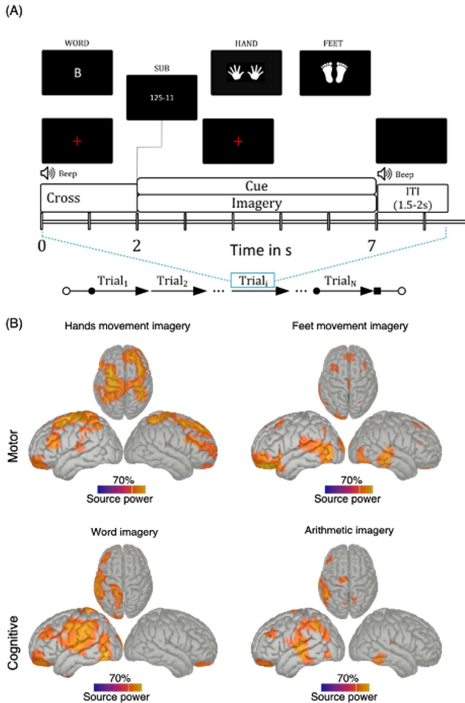
Figure 1. MEG beta-band source activities during BCI task imagery activities in 17 healthy control. (A) Experiment design, (B) group average beta-band, 17-25Hz of 4 tasks source responses.
